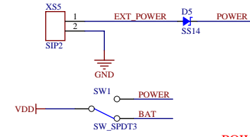
POWER SELECT
